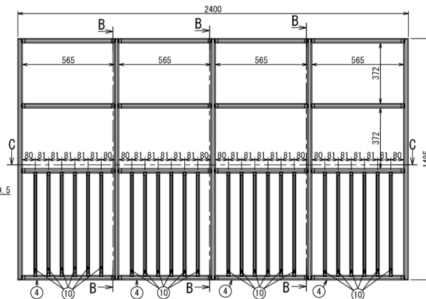
Back View (1:15)
