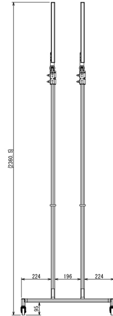
Front View (1 : 12)
