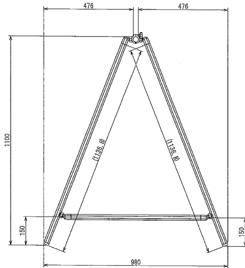
Front View
