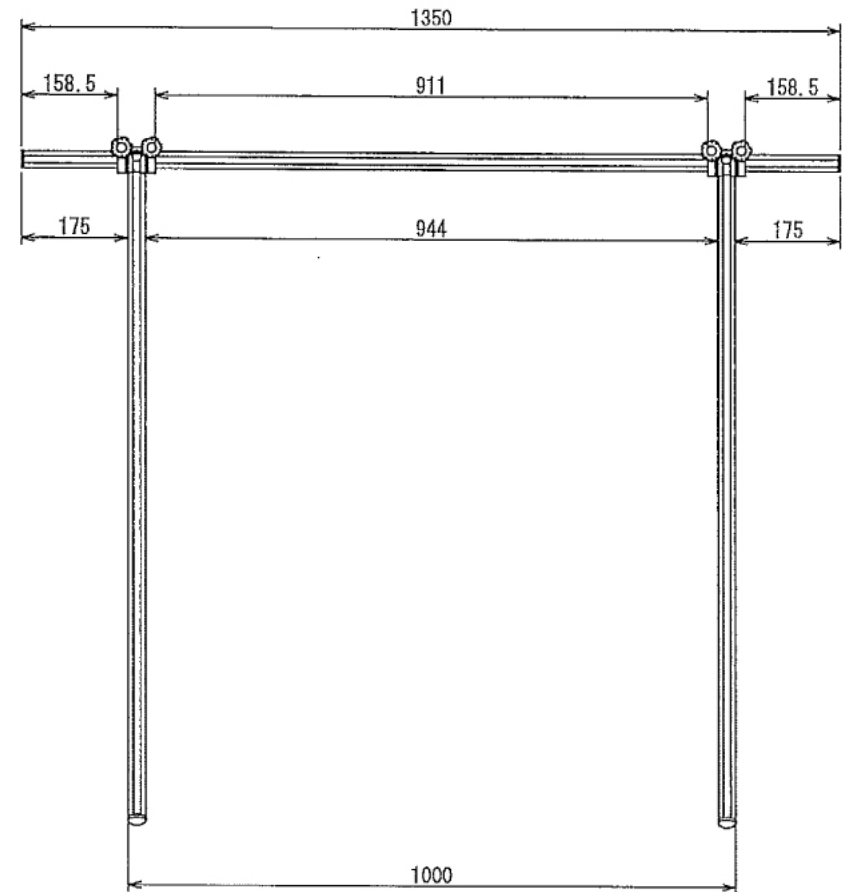
Right View
