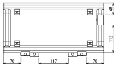
Back View Door A (1:5)
