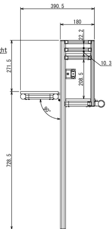
Right View Show All Door Open(1:8)
