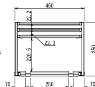
Back View (1:10)
