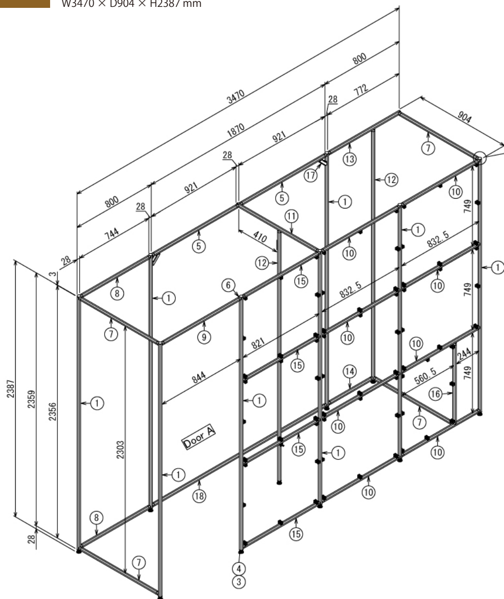
A (1 : 4) Inside of Dimensions
