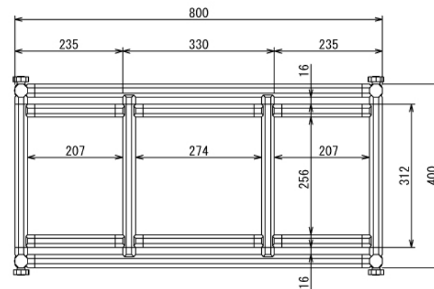
Top View (1:8)
