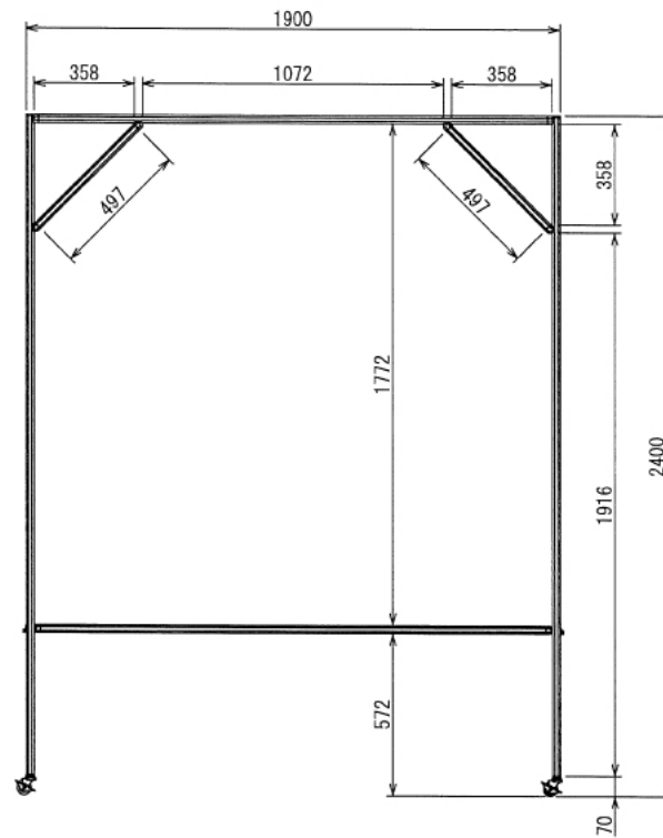
Front View (1:20)
