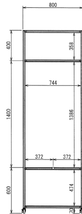
Right View (1:20)
